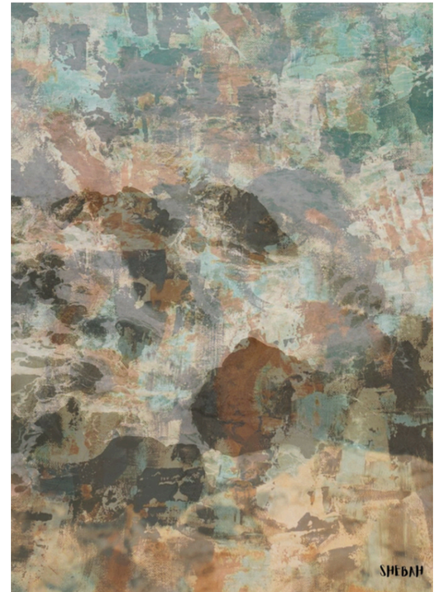
The Earth III
